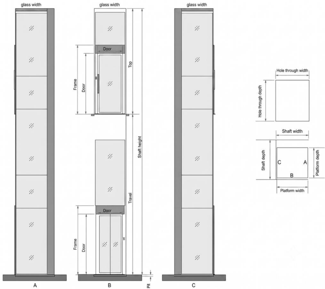
HD Screw Elevator Reserved Dimension Drawing
